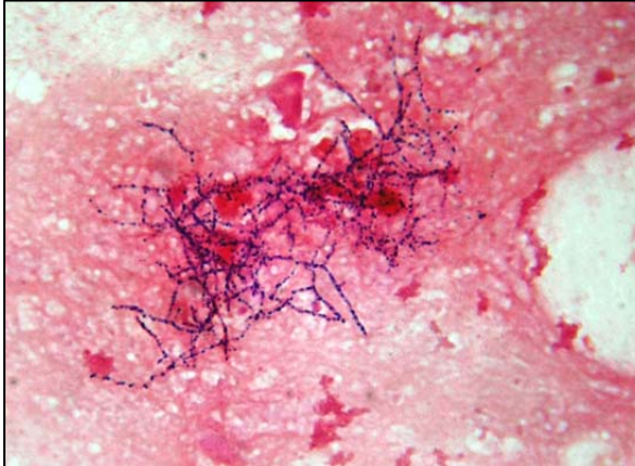
Gram Stain
