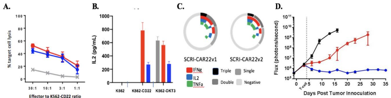
Figure 3-2 Comparison of SCRICAR22v1 and SCRI-CAR22v2.
